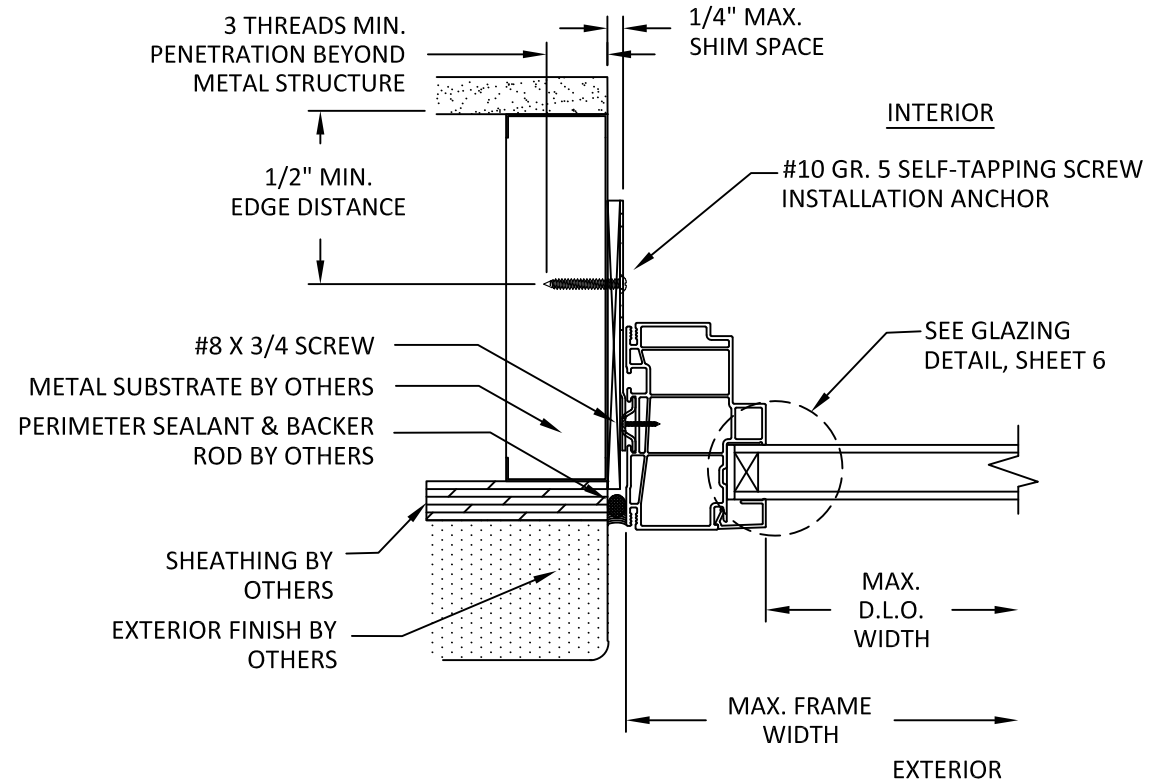
B 5 HORIZONTAL SECTION CLIP INSTALLATION METAL SUBSTRATE
